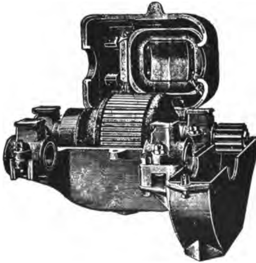
FIG. 484.—A Heavy Vehicle or Street-Car Motor, with single reduction, showing working parts in position.
